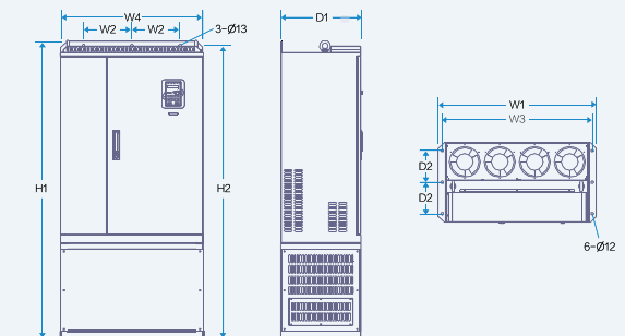
355-500kW Floor mounting Installation diagram
