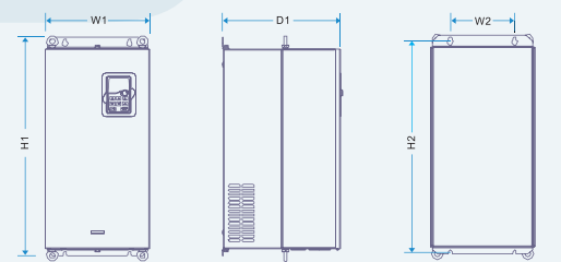
18.5-55kW Installation
