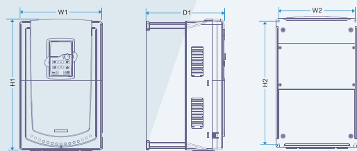
18.5-55kW Installation
